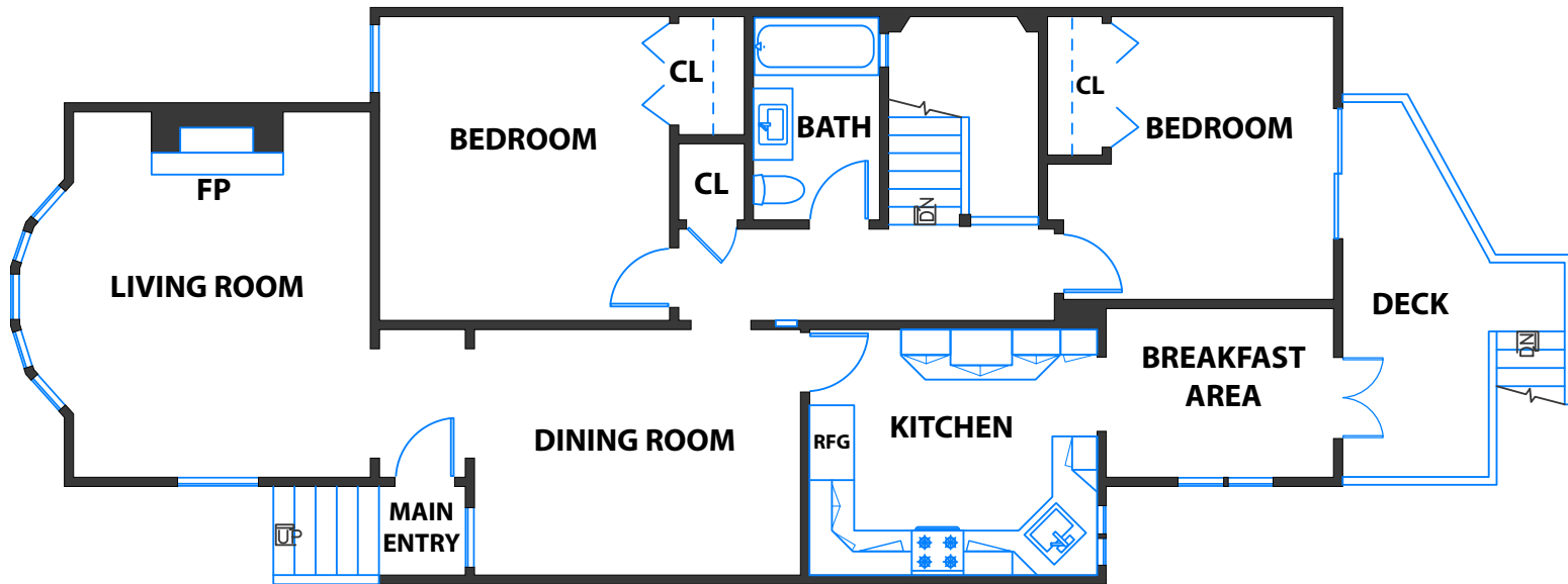
UPPER LEVEL
